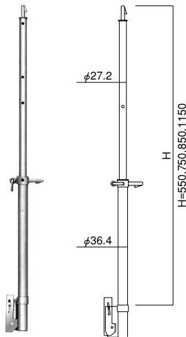
伸縮手摺柱 RT-6...3.5kg
